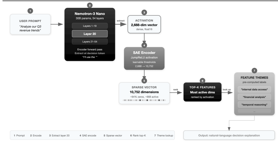
Fig. 5. Inference pipeline for real-time decision explainability. A user prompt is encoded by the Nemotron subject model; the hidden state at layer 20 is intercepted and projected through the trained SAE into a sparse 10,752-dimensional feature vector. The top-K active dimensions are mapped to pre-computed feature labels to produce a human-readable decision report.
