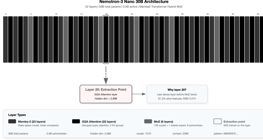
Fig. 3. Architecture of the Nemotron-3-Nano-30B subject model showing all 52 layers. The model interleaves Mamba2 (23 layers), GQA Attention (23 layers), and Mixture-of-Experts (6 layers). Activations are extracted at layer 20, a GQA Attention layer in the mid-network, before the MoE layers that introduce sparse expert routing.
