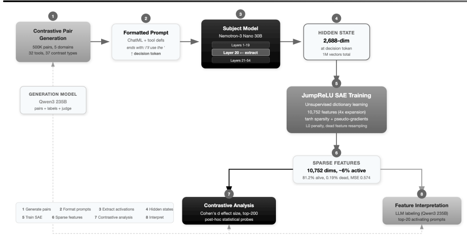
Fig. 1. Overview of the training pipeline. Contrastive pairs are generated and encoded by the subject model. The SAE is trained unsupervised on the extracted activations; contrastive pairs serve only as post-hoc statistical probes for feature analysis and interpretation.
