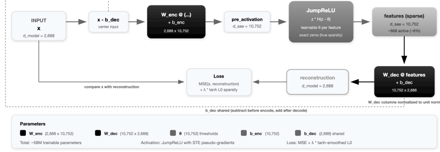
Fig. 4. JumpReLU Sparse Autoencoder architecture. The input activation \mathbf{x} is centered by subtracting \mathbf{b}_{\text{dec}} , projected to a 10,752-dimensional latent space via \mathbf{W}_{\text{enc}} , and sparsified by the JumpReLU activation with learnable thresholds \theta . The decoder reconstructs via \mathbf{W}_{\text{dec}} + \mathbf{b}_{\text{dec}} (shared bias). The loss combines reconstruction MSE with a smooth tanh-based L0 sparsity penalty.
